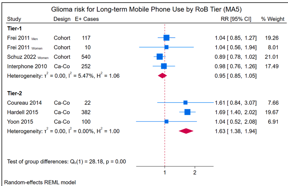
Fig. 4. Meta-analyses of glioma risk in Long-term (TSS 10+ years) mobile phone users stratified on bias-tier (MA1 and MA5 datasets).
